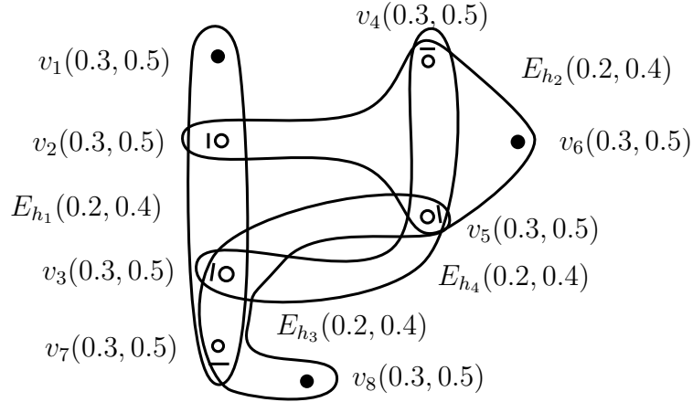
Figure 3. e -Regular and Totally e -regular
