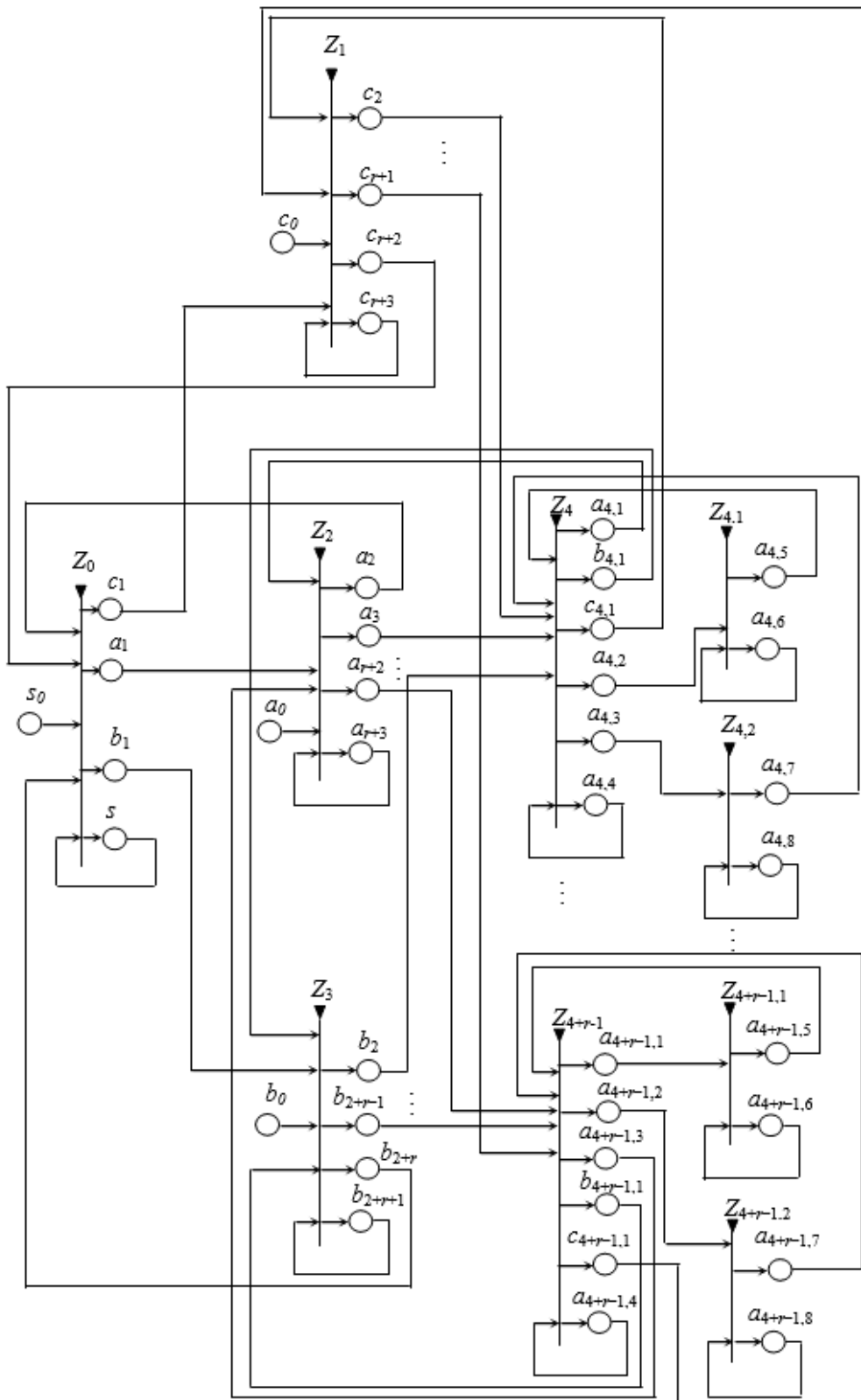
Figure 1. Generalized Net model
